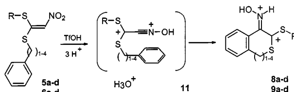
Scheme 2. Formation of cations 8a-d and 9a-d from nitroethylene derivatives 5a-d and 6a-d
