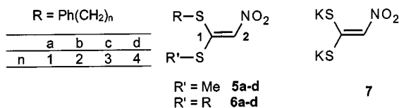
Figure 1. Starting products 5a-d and 6a-d and dipotassium salt 7 used for their synthesis
