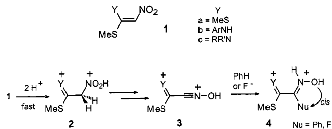
Scheme 1. Reactivity of heterosubstituted nitroethylene derivatives 1 in triflic acid
