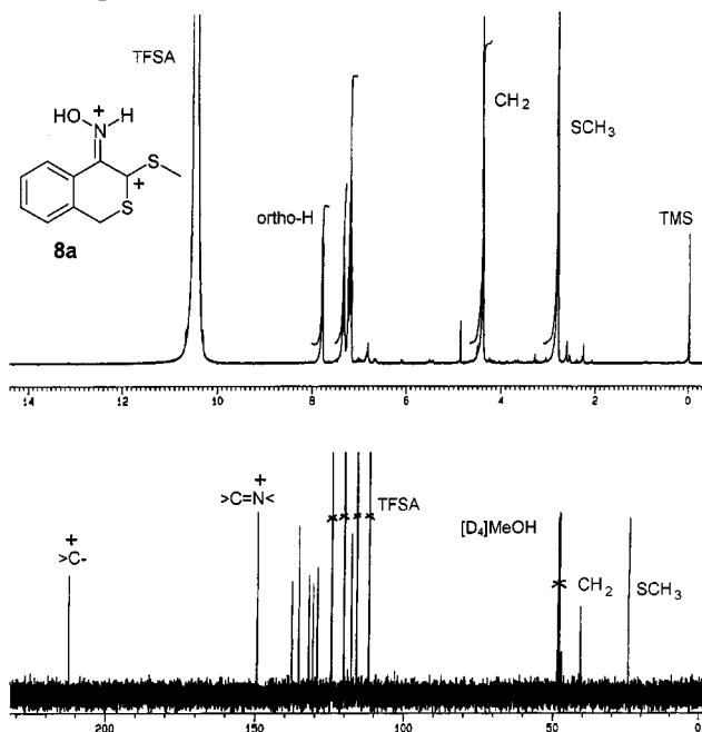
Figure 2. NMR spectra of cyclic cation 8a in trifluoromethanesulfonic acid at room temp. (reference TMS in [D 4 ]methanol)
