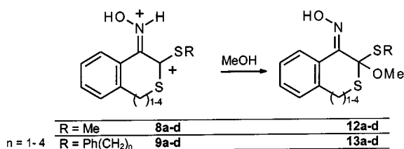
Scheme 3. Trapping of cations 8a–d and 9a–d by methanol
